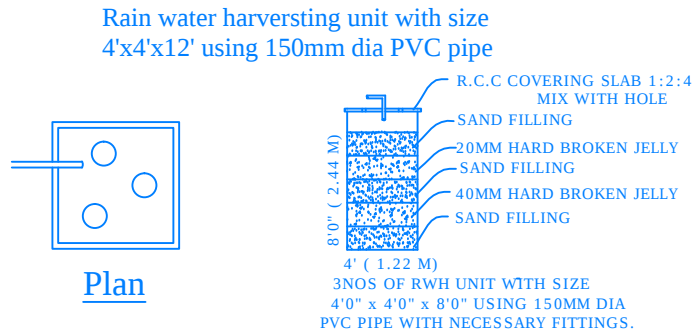
Rain Water Harvesting unit
