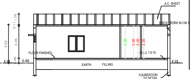
SECTION "A-B"
