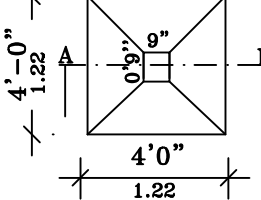
COLUMN DETAILS
