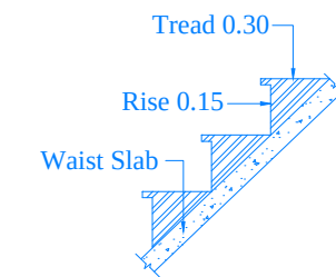
Section of the Staircase Not to scale
