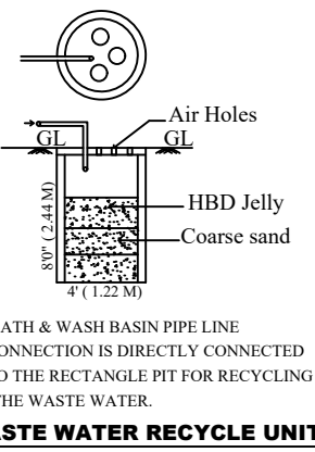
WASTE WATER RECYCLE UNIT
