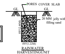
RAINWATER HARVESTING UNIT
