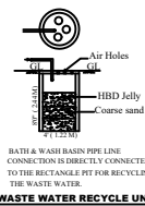
WASTE WATER RECYCLE UNIT
