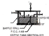
SEPTIC TANK SECTION-XY
