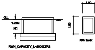
RWH_CAPACITY_L=2000LTRS
