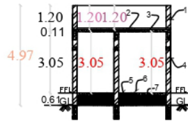
SECTION "A-B"
