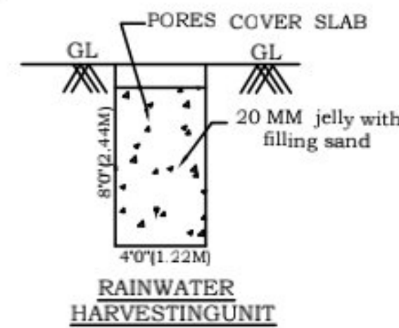
FOUNDATION DETAIL
