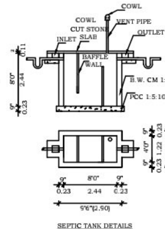
SEPTIC TANK DETAILS
