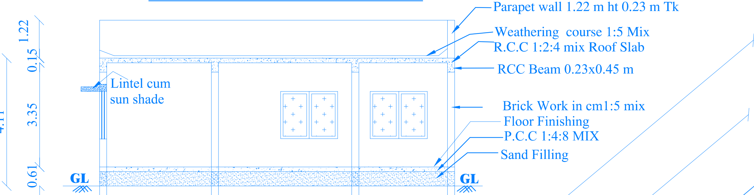
FRONT ELEVATION
