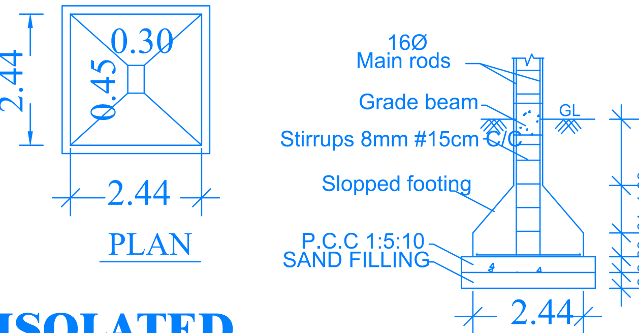
ISOLATED FOOTING (2.44x2.44)
