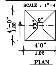
COLUMN DETAILS
