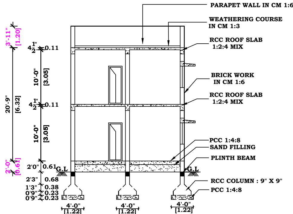
SECTION - KK
