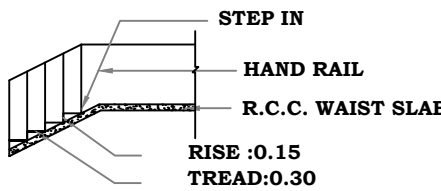
STAIR DETAILS
