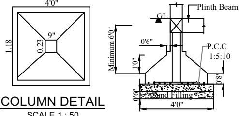
COLUMN DETAIL SCALE 1 : 50
