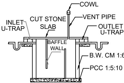
SEPTIC TANK DETAILS SIZE :6'0\"/>
