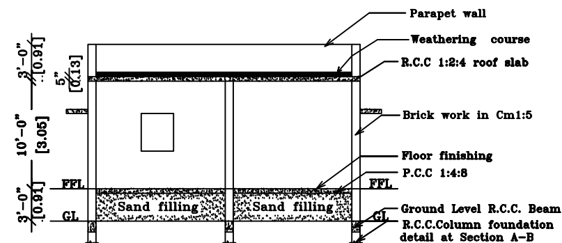
SECTION ON 'A'
