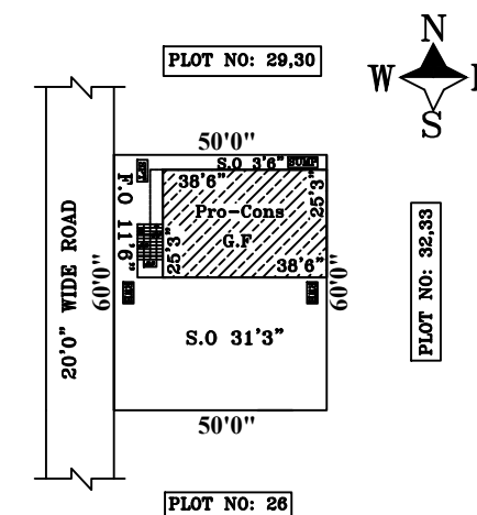
SITE PLAN
