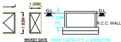
WICKET GATE RWHTANK_CAPACITY_L=2000LTRS
