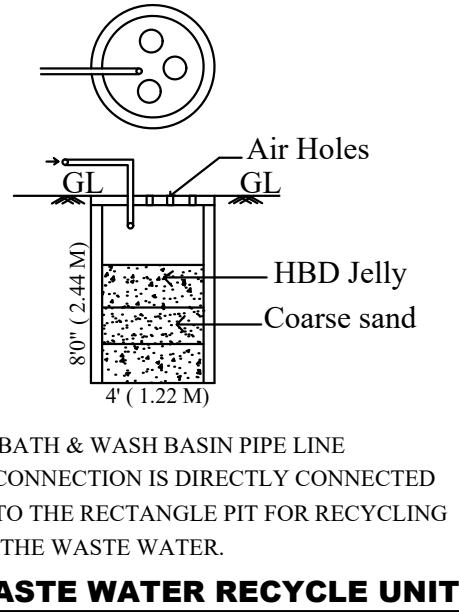
WASTE WATER RECYCLE UNIT
