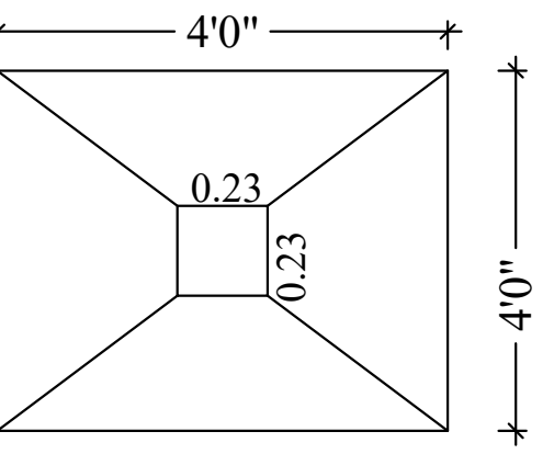
FOOTING / COLUMN DETAIL
