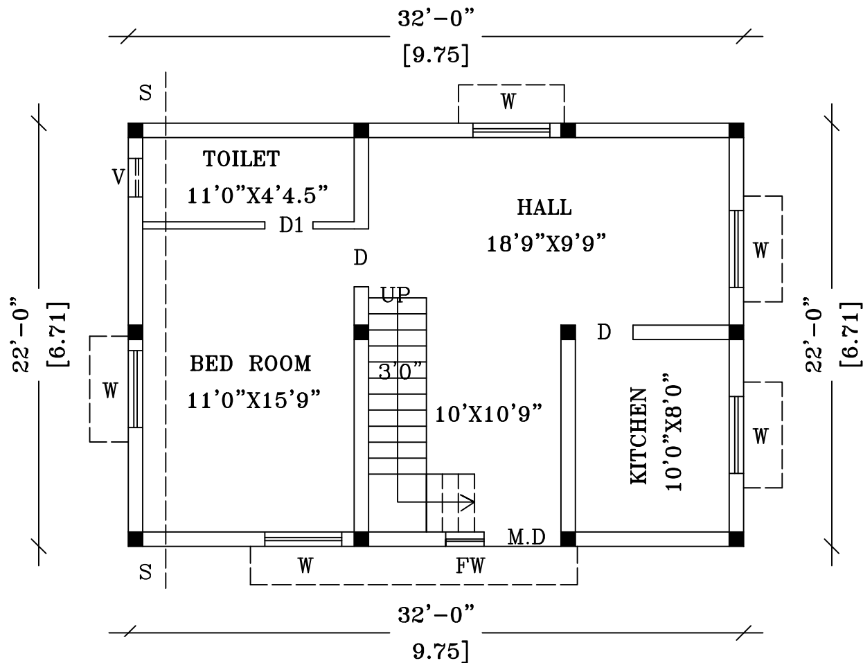
FLOOR PLAN
