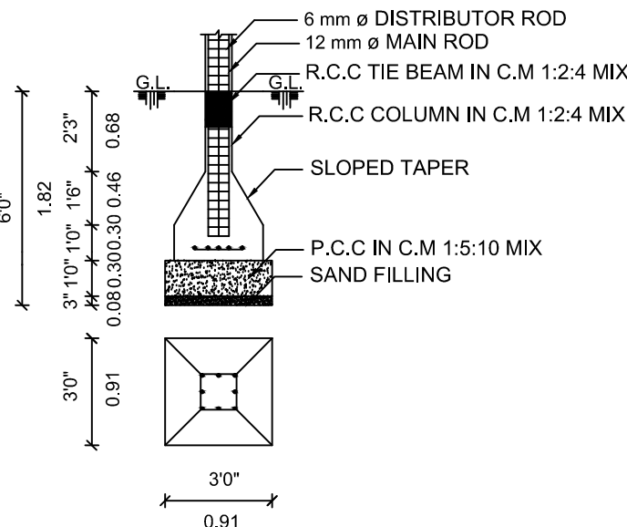
COLUMN IN FOUNDATION
