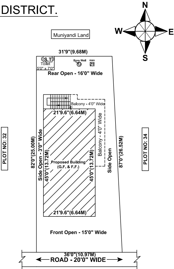
SITE PLAN
