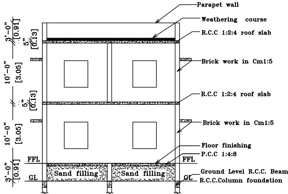
SECTION ON 'SJ'
