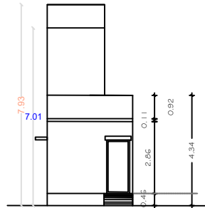
FRONT ELEVATION
