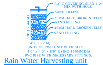
Rain Water Harvesting unit
