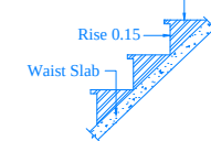
Section of the Staircase Not to scale
