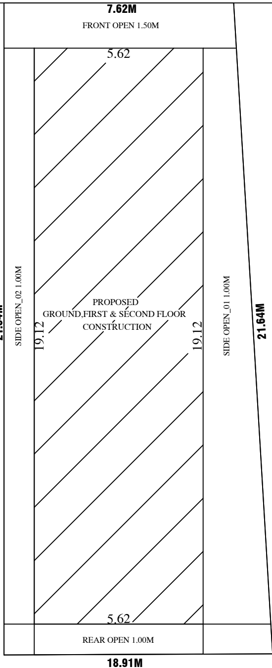
SITE PLAN
