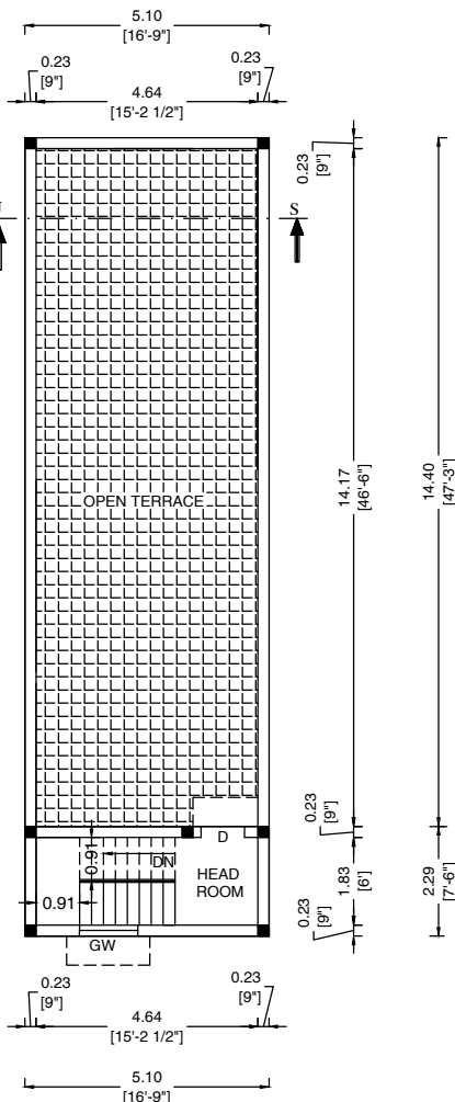
PRO., TERRACE FLOOR PLAN
