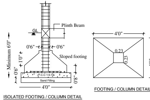
COLUMN DETAILS
