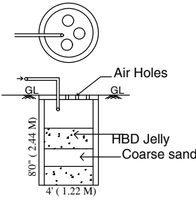
RAIN WATER HARVESTING TANK DETAIL
