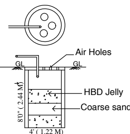
WASTE WATER RECYCLE UNIT
