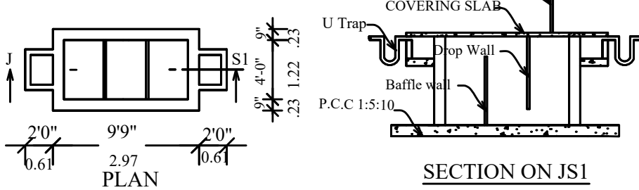
SECTION ON JS1
