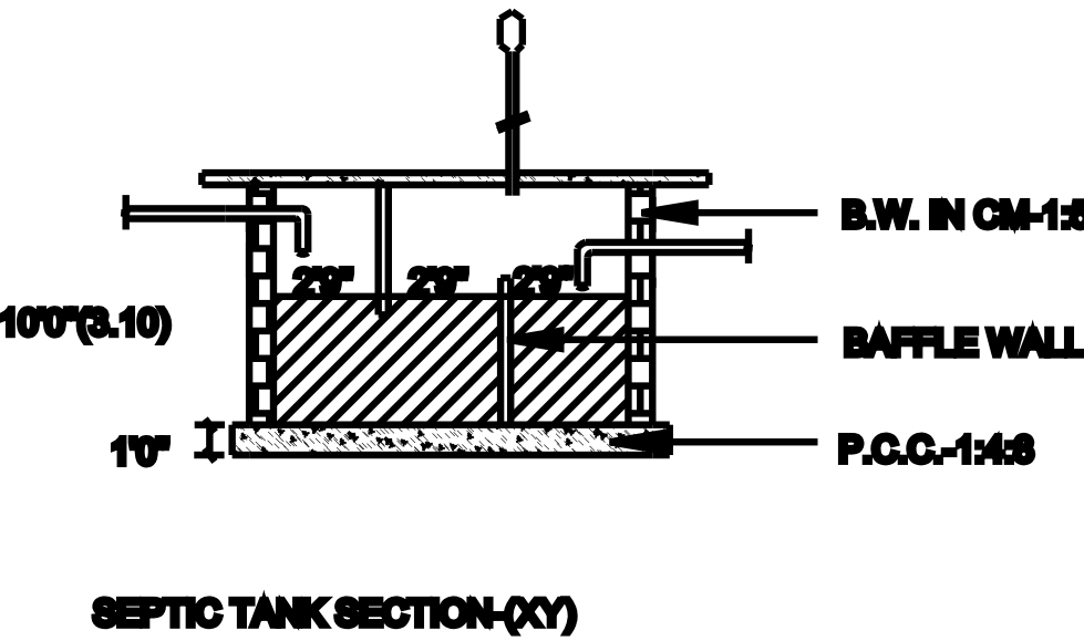
SEPTIC TANK SECTION-QC1
