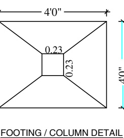
FOOTING / COLUMN DETAIL
