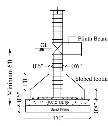
ISOLATED FOOTING / COLUMN DETAIL
