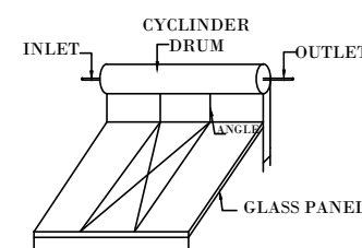
SOLAR ENERGY (NOT TO SCALE)
