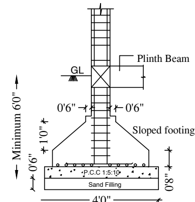
ISOLATED FOOTING / COLUMN DETAIL
