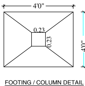
FOOTING / COLUMN DETAIL
