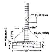
ISOLATED FOOTING / COLUMN DETAIL
