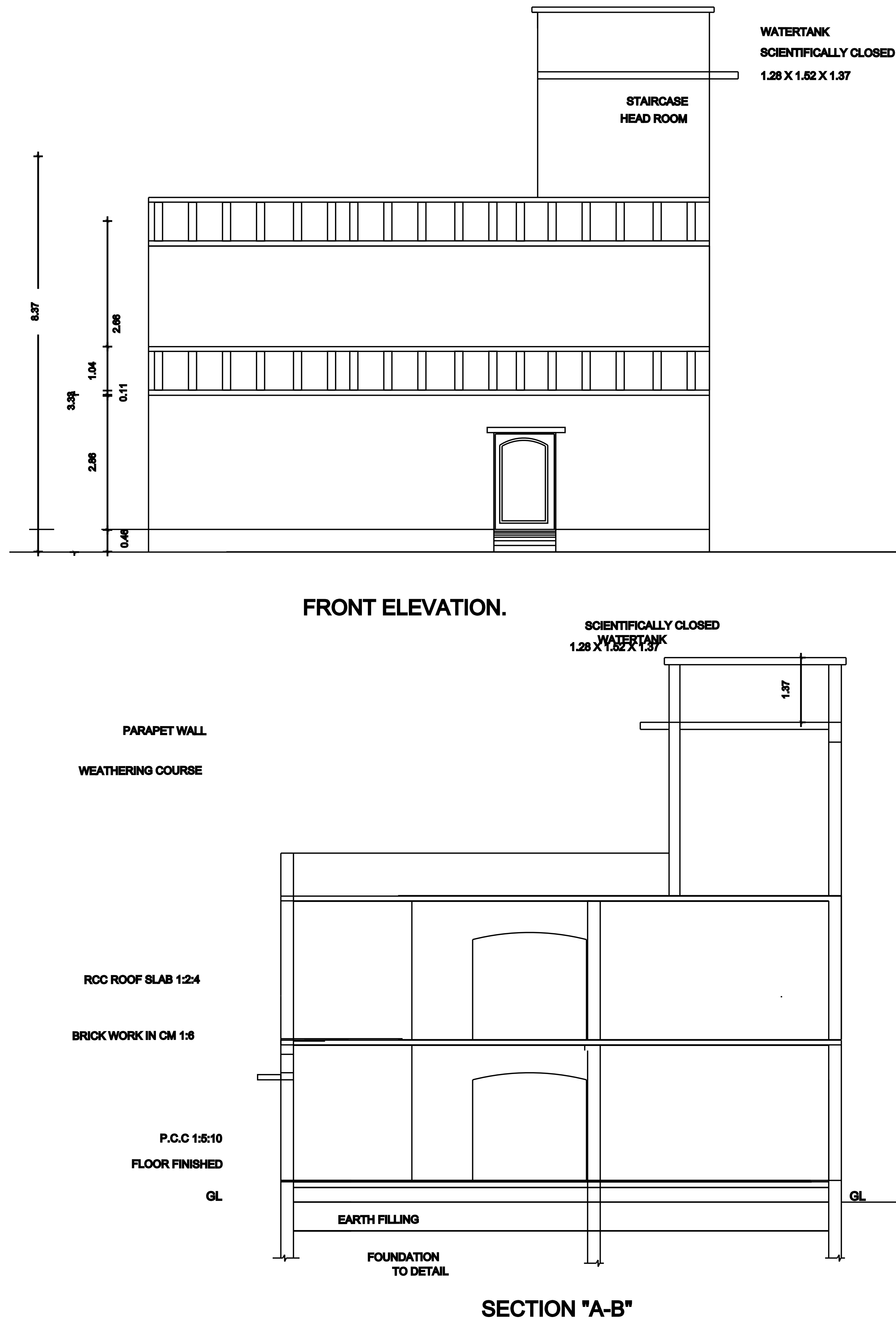
SECTION "A-B"
