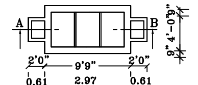
SEPTIC TANK DETAILS
