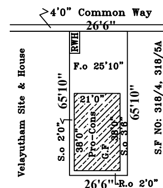
SITE PLAN SCALE: 1INCH=33FEET
