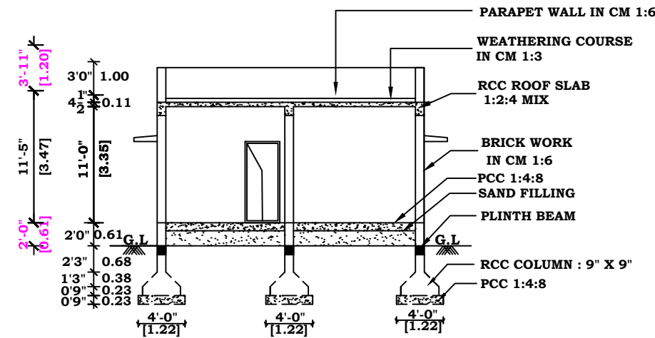
SECTION - KK
