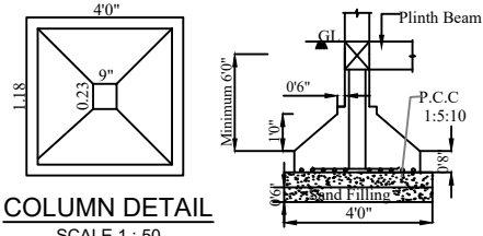
COLUMN DETAIL
