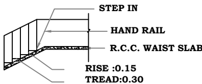
STAIR DETAILS
