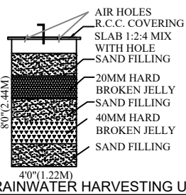
RAINWATER HARVESTING UNIT
