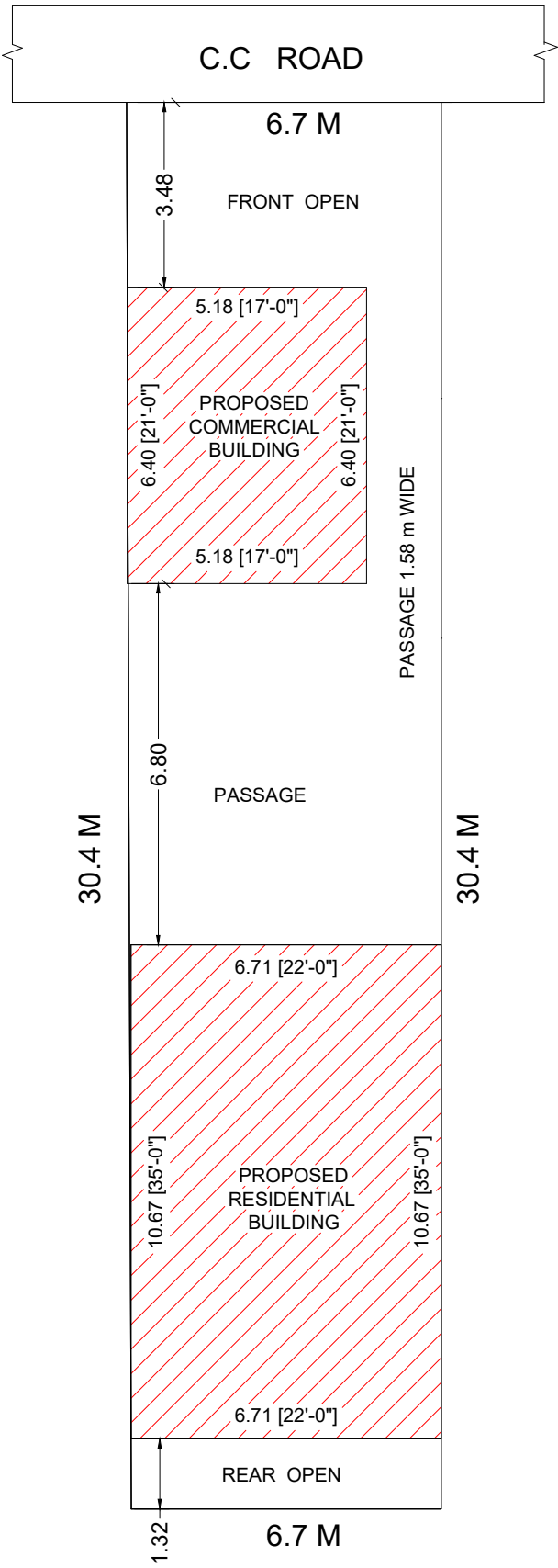
SITE PLAN
