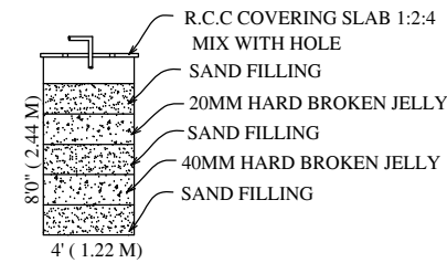
Waste Water Recycle Unit Not To Scale
