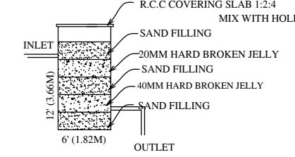
Waste Water Recycle Unit Not To Scale
