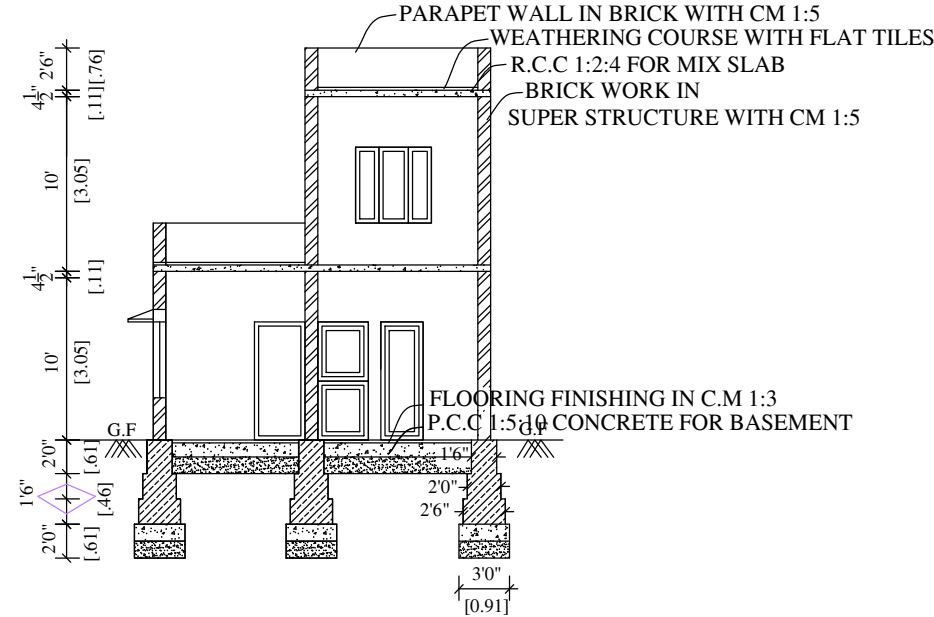
SECTION NO R-S
