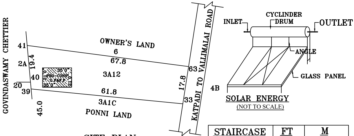
SITE PLAN
