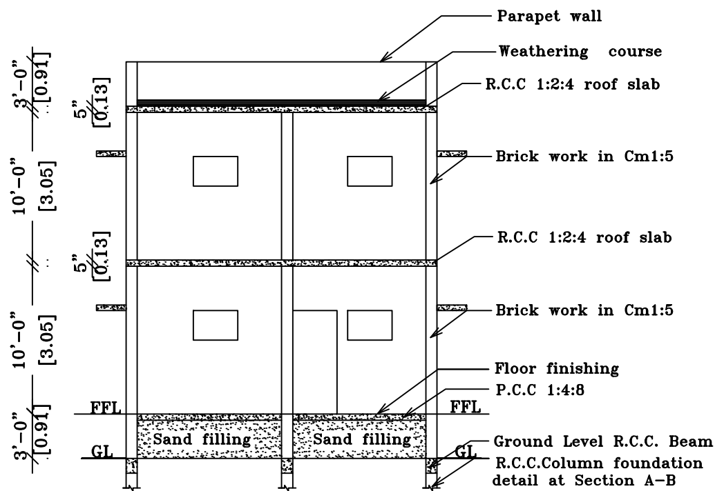
SECTION ON 'SA'
