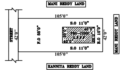
SITE PLAN
