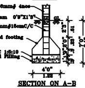
SECTION ON A-B
