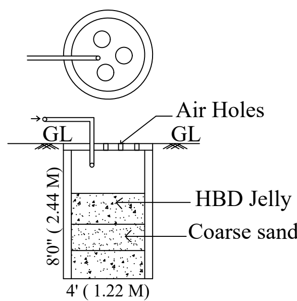
RAIN WATER HARVESTING TANK DETAIL
