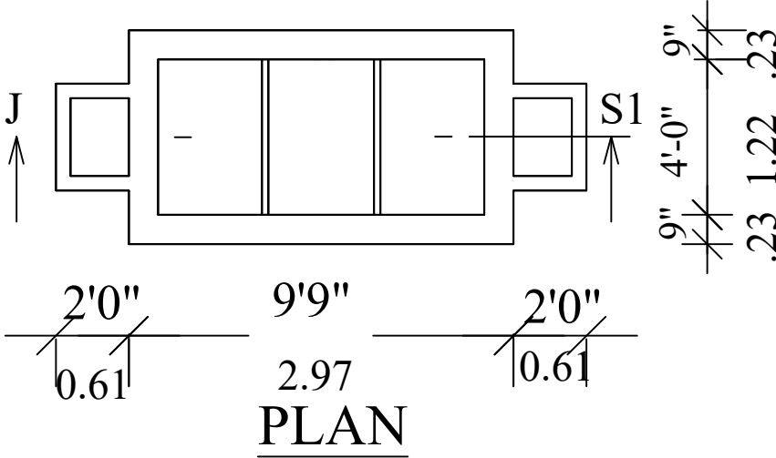
ISOLATED FOOTING / COLUMN DETAIL
