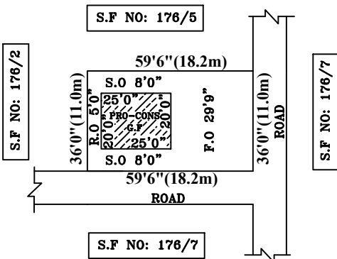
SITE PLAN
