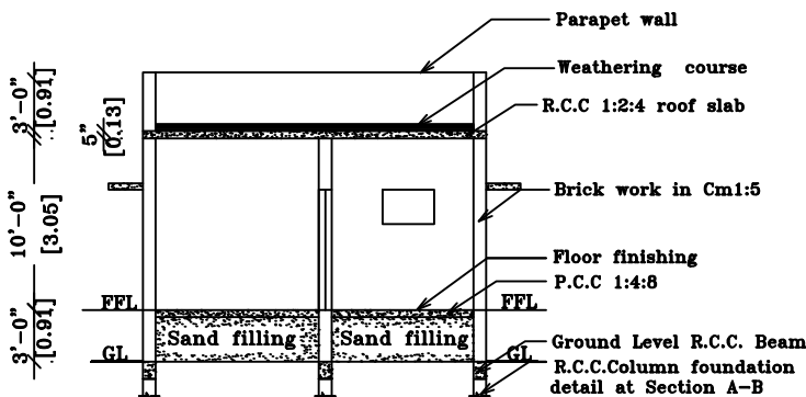
SECTION ON 'SA'
