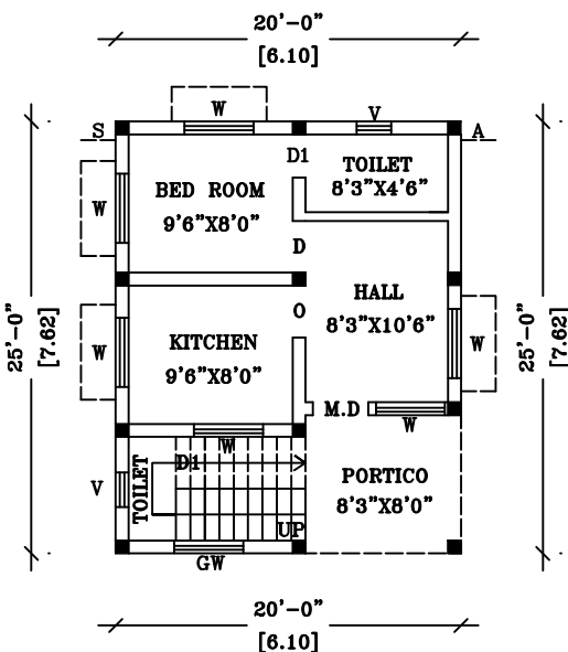
ROUND FLOOR PLAN
