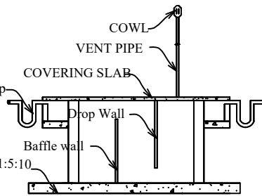
SECTION ON JS1
