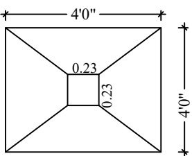
FOOTING / COLUMN DETAIL
