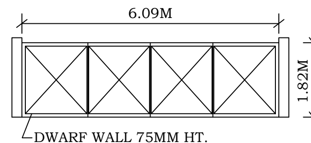
MAIN GATE ELEVATION
