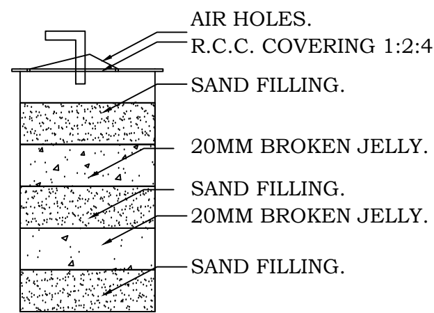
RAIN WATER UNITS
