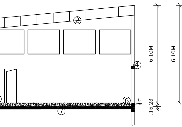
SECTION ON 'CY'
