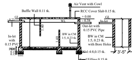
Section - Septic tank & Soak pit
