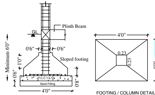
COLUMN DETAILS
