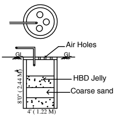
WASTE WATER RECYCLE UNIT
