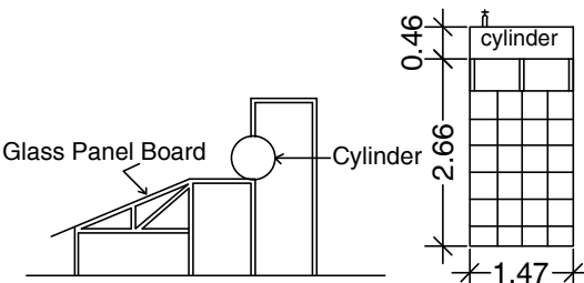
SOLAR ENERGY SYSTEM
