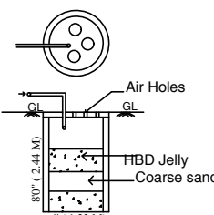
RAIN WATER HARVESTING TANK DETAIL
