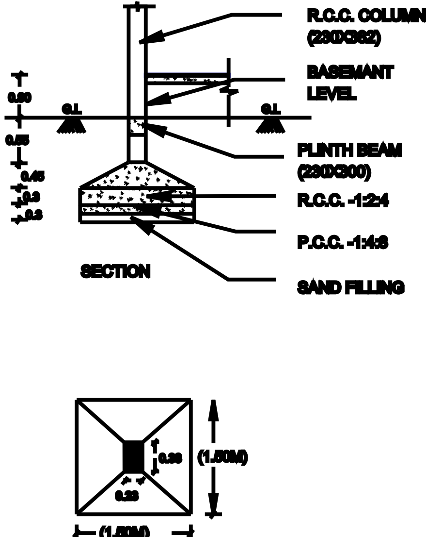
DETAILS OF COLUMN FOUNDATION
