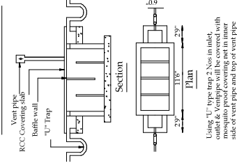
Septic tank with "U" Trap (NTS)
