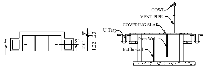
SECTION ON JS1
