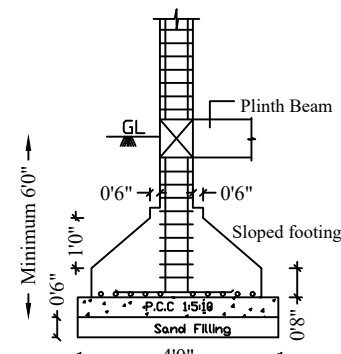
ISOLATED FOOTING / COLUMN DETAIL
