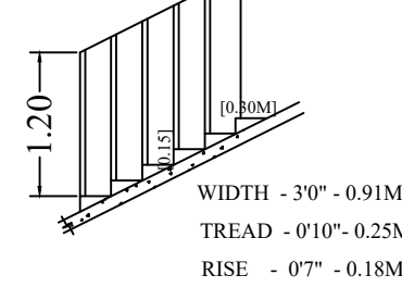
STAIRCASE DETAILS
