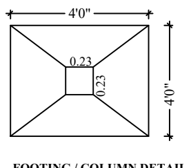
FOOTING / COLUMN DETAIL
