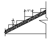
Staircase Detail
