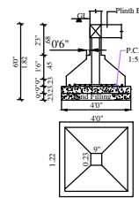
COLUMN DETAIL
