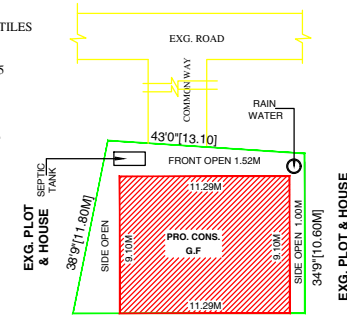
SITE PLAN
