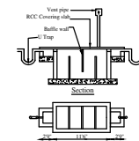
Septic Tank With U Trap
