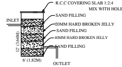
Waste Water Recycle Unit
