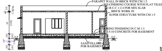
SECTION NO R-S
