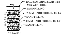
Rain Water Harvest Unit
