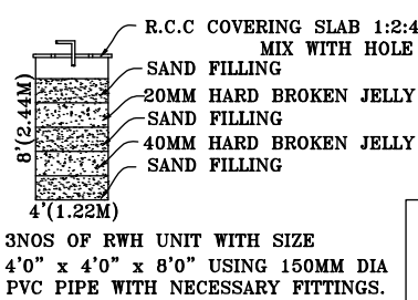
RAIN WATER HARVEST UNIT
