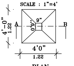
COLUMN DETAILS
