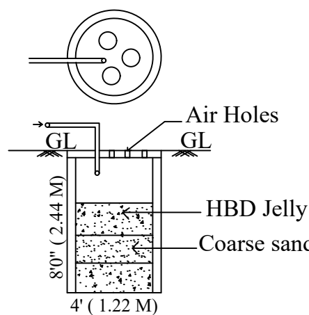
RAIN WATER HARVESTING TANK DETAIL
