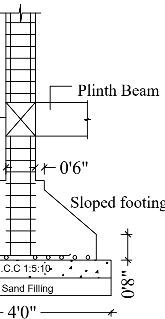
ISOLATED FOOTING / COLUMN DETAIL
